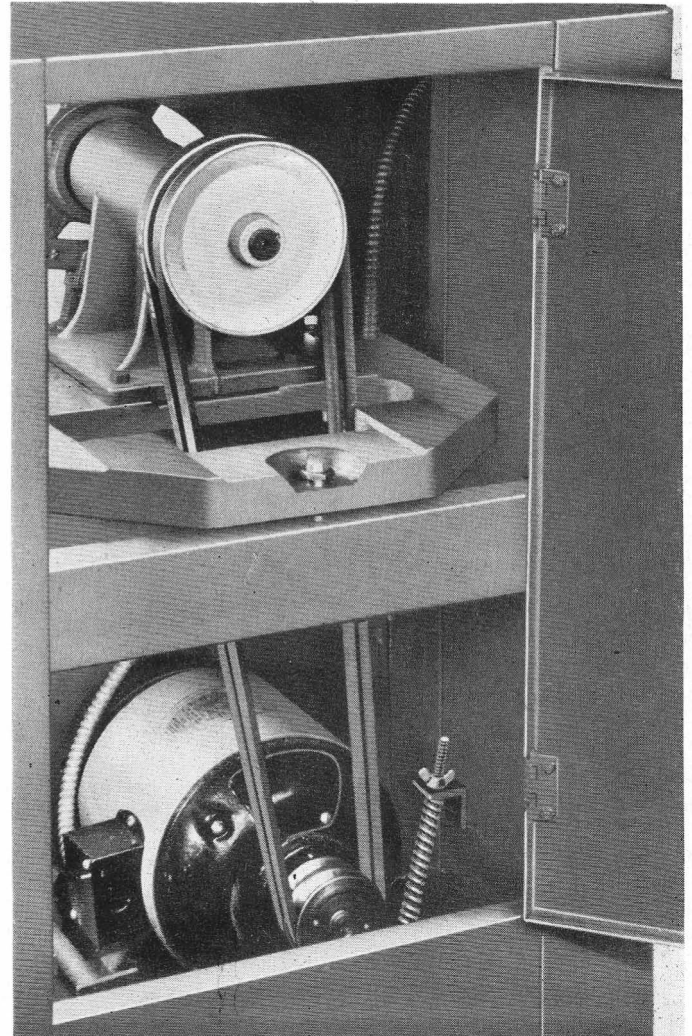
Fig. 6. V-Belt Drive.
