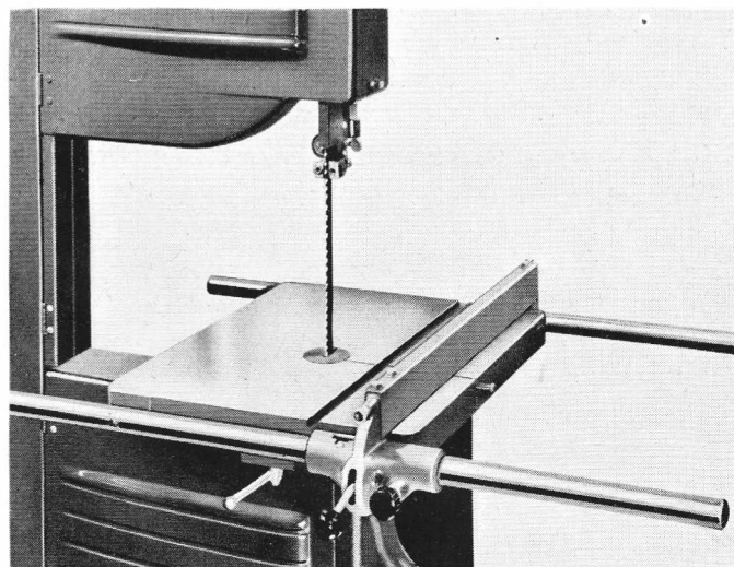
Fig. 20. Rip Fence Mounted on Table.
