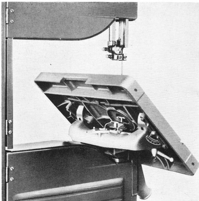
Fig. 12. Table Tilted to Right, Showing Trunnions and Stop Bar.
