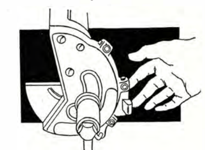
On our fence, once the stops at 45 and 90 degrees have been set, there is never again any necessity to use the square or bevel. A flip of the finger takes the stop out of the way for tilting.
