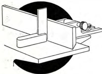
Due to the absence of stops on old-type fences, the square must be used to re-set the fence vertically every time the fence is tilted.
