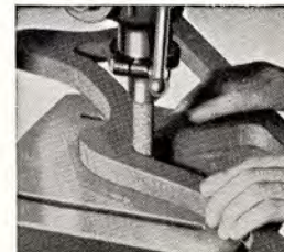
Sanding the edges of carved work with the sanding drum saves hours of tedious labor.
