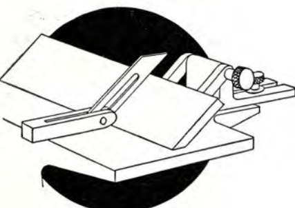
On old-type fences, it is also necessary to use a bevel gage or other angle gage every time the fence must be set to 45 degrees for miter work.
