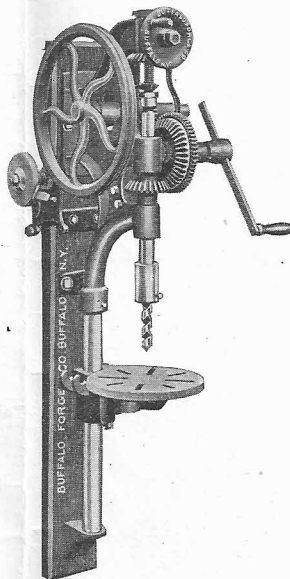
No. 74 DRILL.
