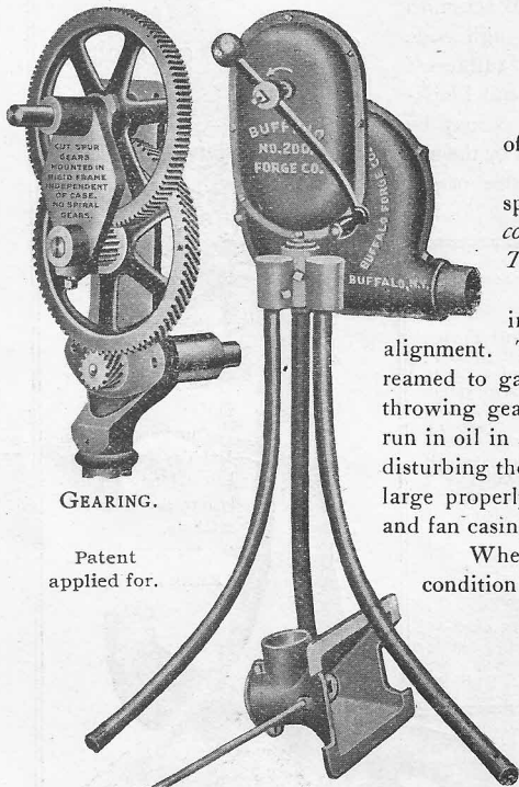
BUFFALO No. 200 BLOWER With No. HH Tuyere.
