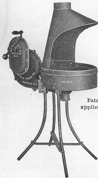
No. 626 FORGE.
