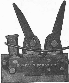
BUFFALO No. 1 TIRE UPSETTER.
