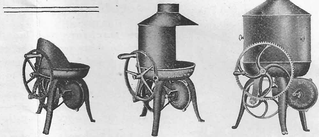
BENCH FORGE, No. 7. BENCH FORGE, No. 8. BENCH FORGE, No. 9.
