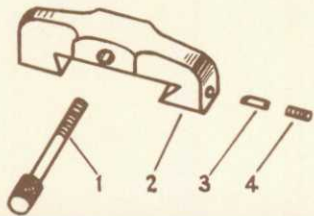
9" & 10-K THREAD CUTTING STOP
