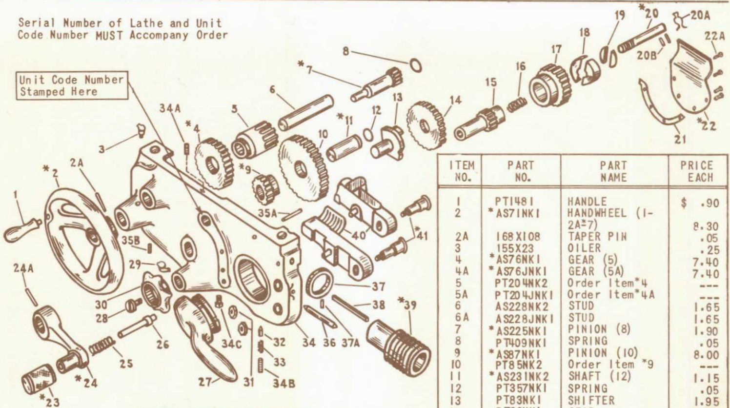
9" & 10-K APRON Model A & B
