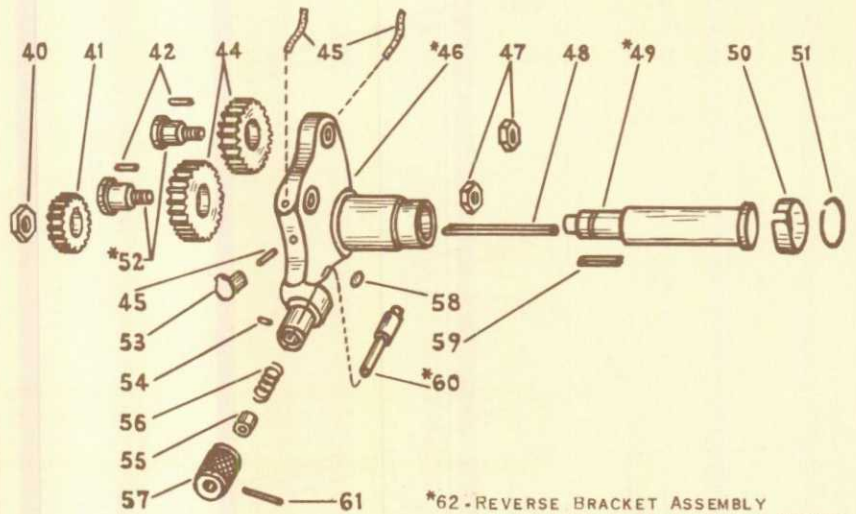
REVERSE BRACKET ASSEMBLY
