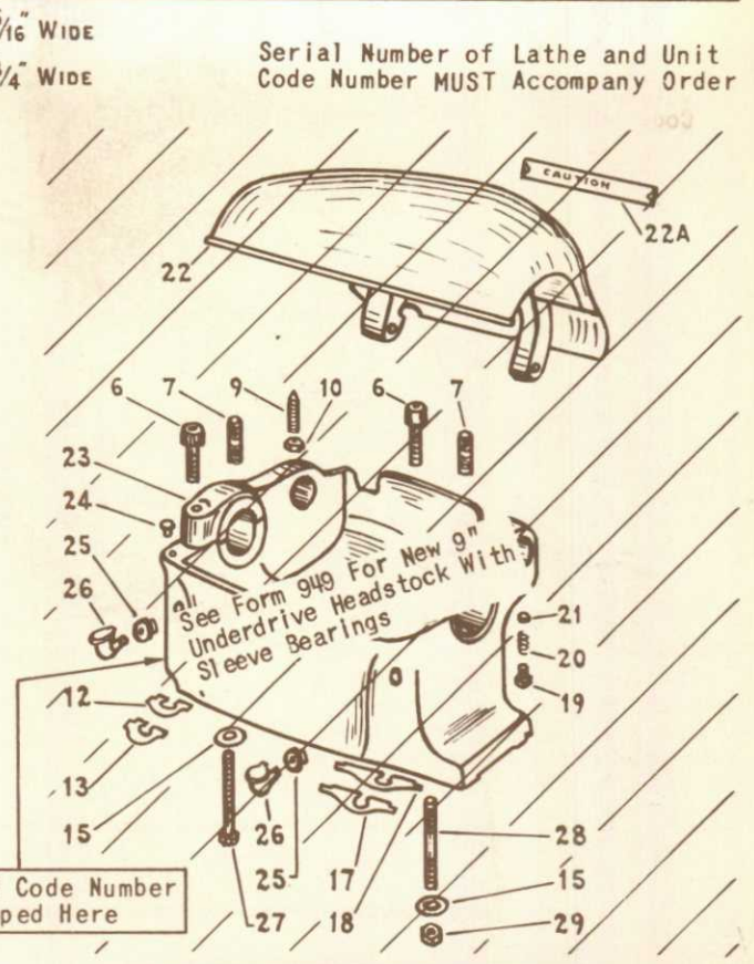
9" UNDERDRIVE HEADSTOCK Model A, B, & C
