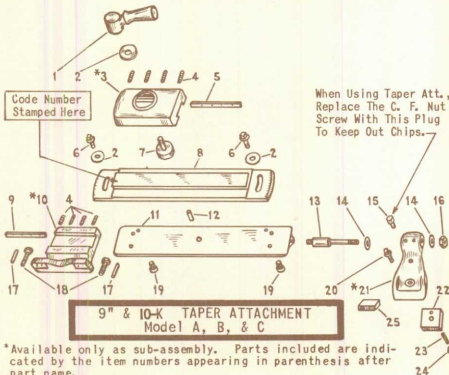
9" HANDLEVER COLLET ATTACHMENT Model A, B, & C
