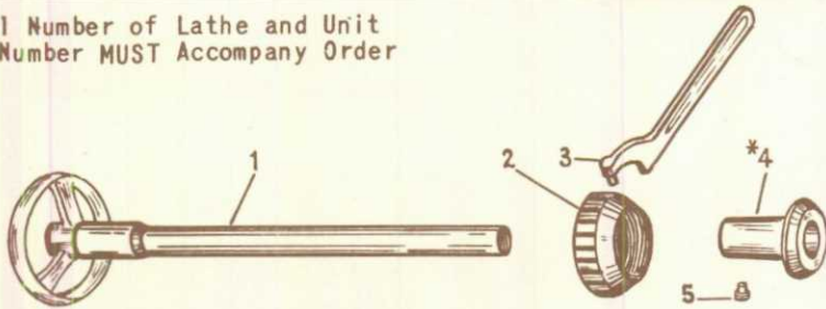
9" HANDWHEEL COLLET ATTACHMENT Model A, B, & C
