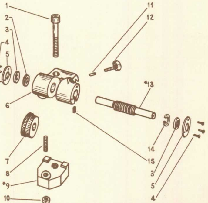
9" & 10-K MICROMETER CARRIAGE STOP
