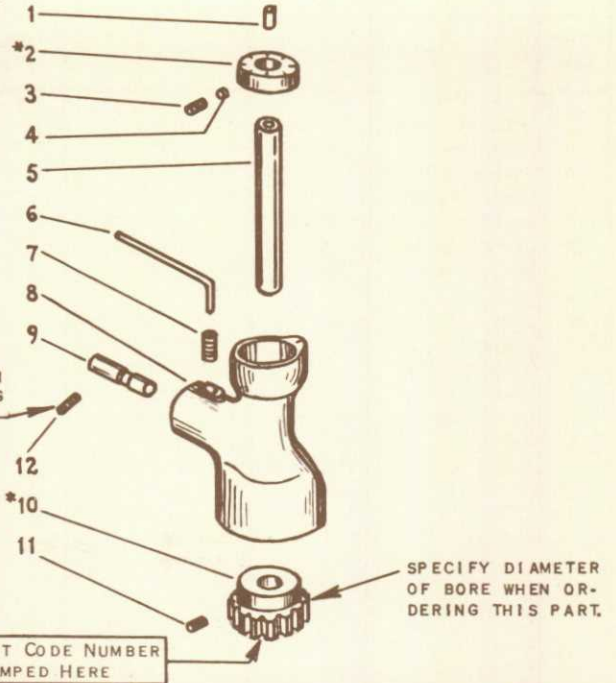
9" & 10-K THREAD DIAL INDICATOR
