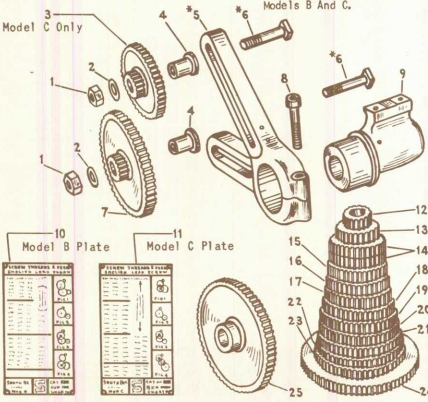
9" & 10-K STANDARD CHANGE GEAR Model B & C
