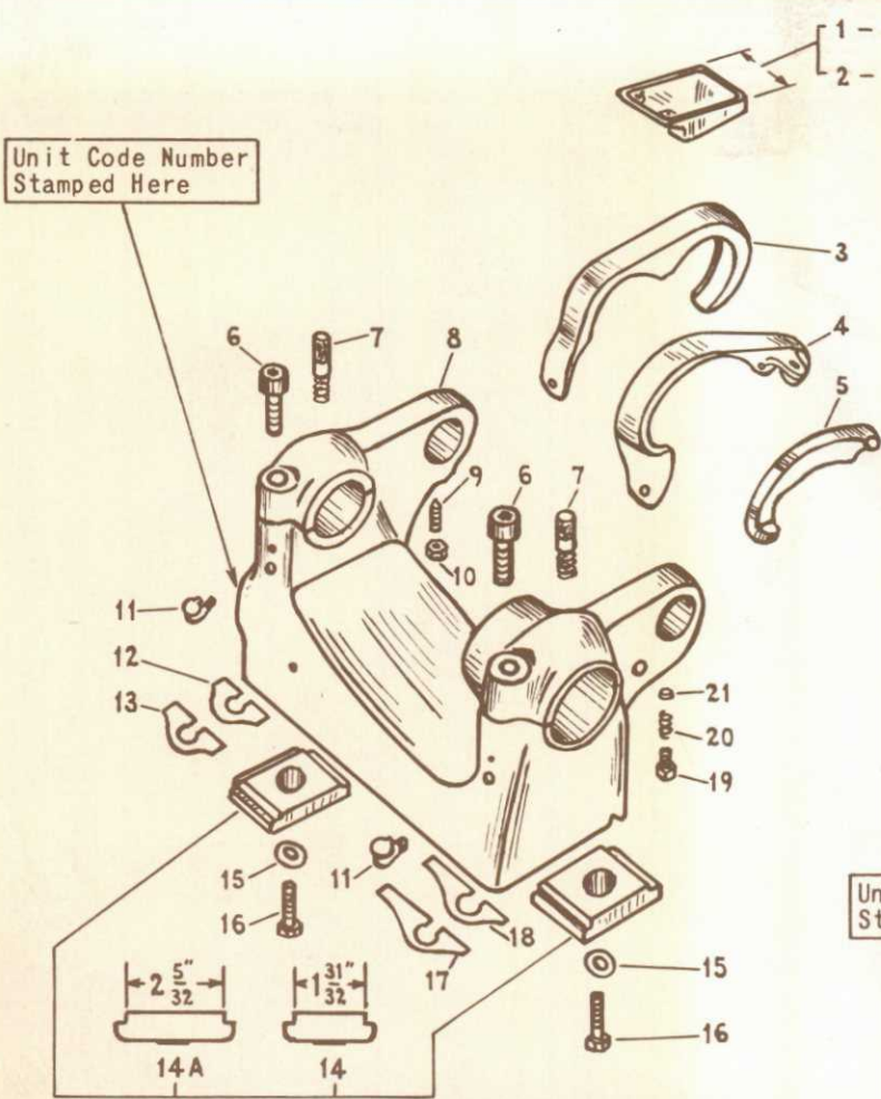
9" HORIZONTAL DRIVE HEADSTOCK Model A, B, & C
