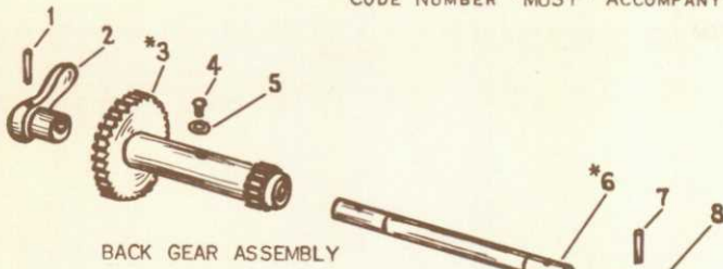
BACK GEAR ASSEMBLY
