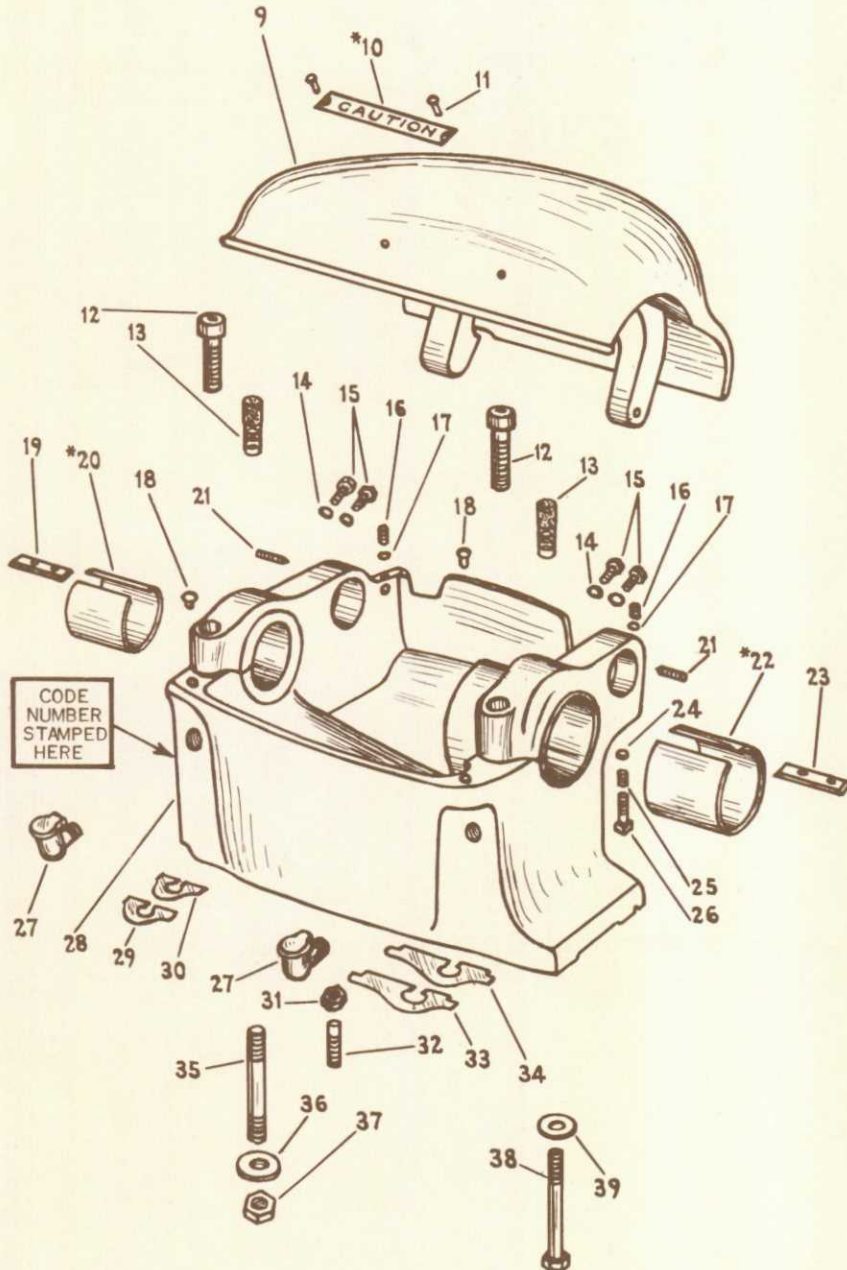
9" UNDERDRIVE HEADSTOCK WITH SLEEVE BEARINGS MODEL A, B, OR C
