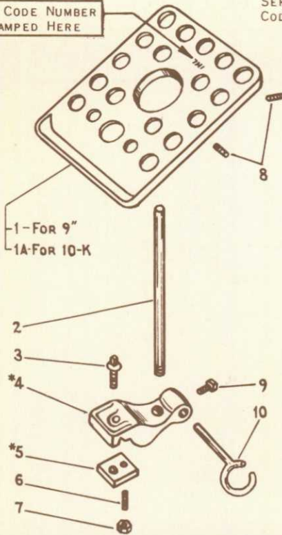
9" & 10-K COLLET RACK
