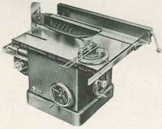
Model No. 85A 8" TILT ARBOR SAW
