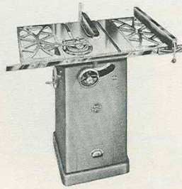
Model No. 60 9" TILT ARBOR SAW
